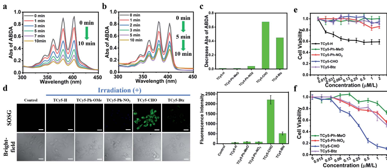
Fig. 3 Time-dependent UV-vis absorption spectra for 9,10-anthracenediyl-bis(methylene)-dimalonic acid (ABDA) over (a) TCy5-CHO and (b) TCy5-Btz under 10 mW \text{cm}^{-2} LED light irradiation in ultrapure water. (c) Decrease in the absorbance value of ABDA at 380 nm under NIR LED irradiation. (d) Fluorescence images of MCF7 cells containing TCy5 (5 \mu\text{M} )/SOSG (10 \mu\text{M} ), indicating the ^1\text{O}_2 generation of TCy5 dyes upon 660 nm light irradiation with a 20 \text{J cm}^{-2} light dose; for SOSG, emissions are collected at 500–580 nm ( \lambda_{\text{ex}} = 488 \text{ nm} ). Scale bar = 20 \mu\text{m} . (e) Dark toxicity effect of TCy5 compounds on MCF7 cells. (f) Phototoxicity effect of four TCy5 compounds on MCF7 cells under 10 mW \text{cm}^{-2} light irradiation for 10 min.
