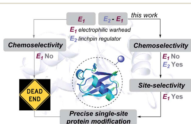
Fig. 1 Lynchpin ( E_2 ) can empower a promiscuous electrophile ( E_1 ) to enable site-selectivity and deliver precise modification of proteins.
