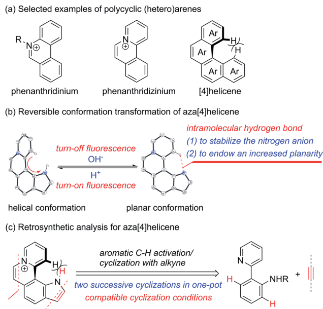
Scheme 1 (a) Selected examples of polycyclic (hetero)arenes. (b) Reversible conformation transformation of aza[4]helicene. (c) Retrosynthetic analysis for aza[4]helicene.
