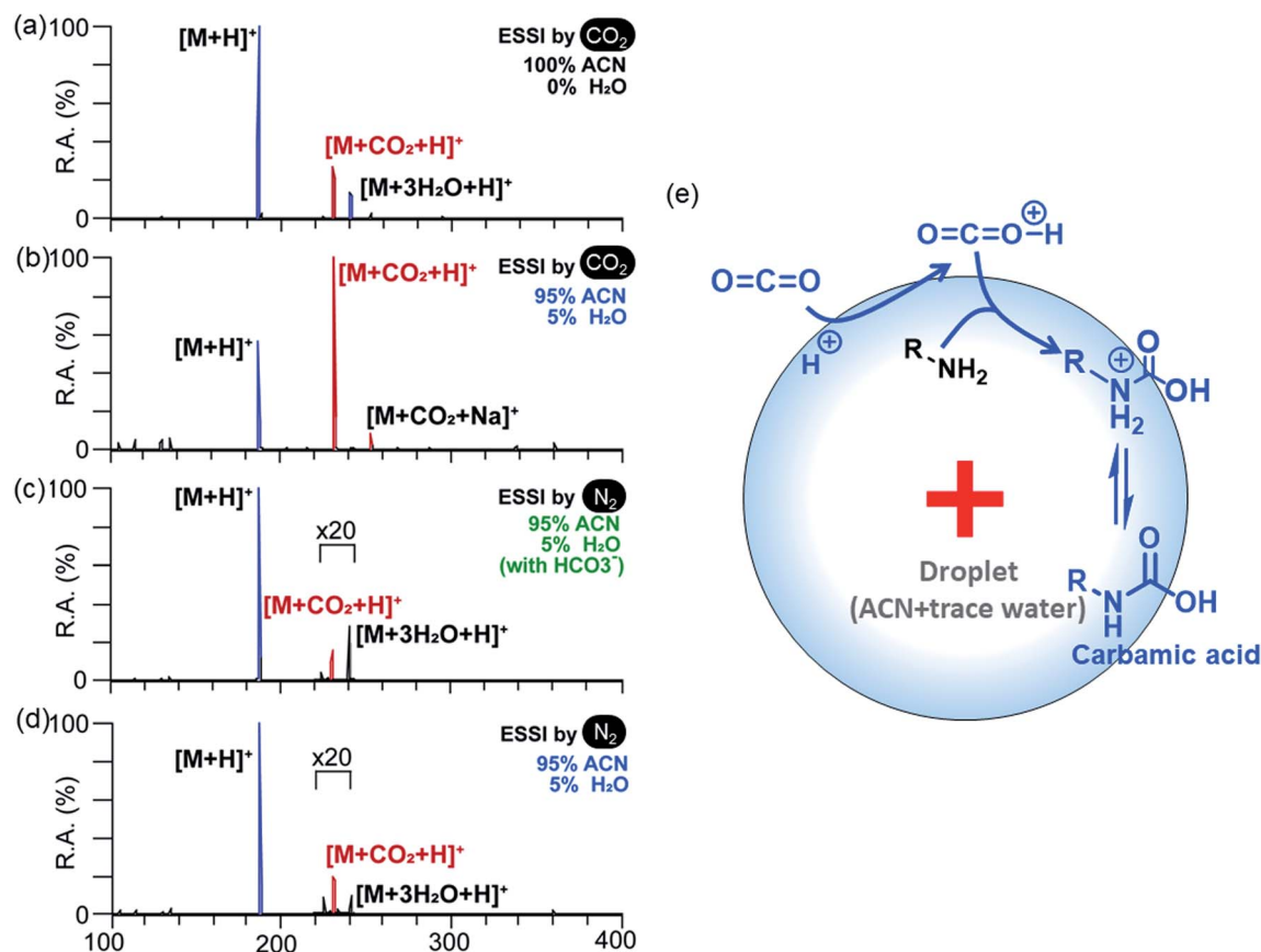
Fig. 3 Droplet reaction showing positive ion ESI mass spectra of (a) ACN droplets and (b) 5% water in ACN droplets with interfacial \text{CO}_2 (c) 5% water in ACN droplets with bicarbonate (added) and (d) droplet reaction of 5% water in ACN droplets with room \text{CO}_2 . (e) Mechanistic description of room air \text{CO}_2 /amine droplet reaction (ACN with small amounts of water). Autoionization at the charged interface gives superacid which protonates \text{CO}_2 , allowing reaction with amine to form the carbamic acid, the protonated form of which is observed at m/z 231 in the mass spectrum.
