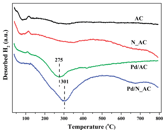
Fig. 5 H 2 -TPD profiles of AC, N_AC, Pd/AC and Pd/N_AC.
