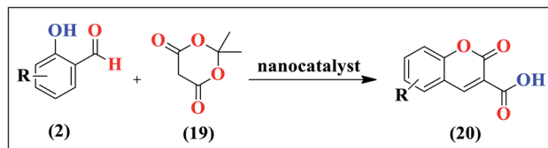
Scheme 17 Synthesis of substituted coumarins.
