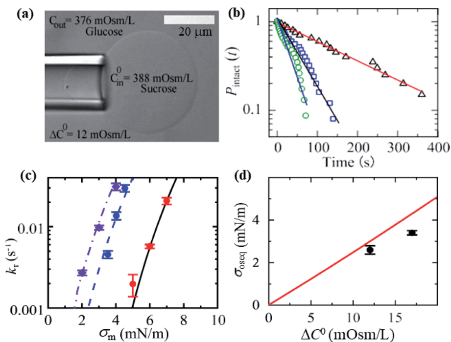
Fig. 15 Constant-mechanical-tension ( \sigma_m )-induced rupture of 40%DOPG/60%DOPC-GUVs in the presence of various osmotic pressures ( \Pi ). (a) A differential interference contrast microscopic image of a GUV aspirated using a micropipette at \sigma_m = 3.5 mN m -1 and \Delta C^0 = 12 mOsm L -1 . (b) The time course of P_{\text{intact}}(t) at tensions \sigma_m of 3.5 ( \Delta ), 4.0 ( \square ), and 4.5 ( \circ ) mN m -1 under \Delta C^0 = 12 mOsm L -1 . The number of GUVs examined was 20–25 in each experiment. The solid lines represent the best fit curves using eqn (4). (c) The \sigma_m -dependent k_r values in the presence of \Delta C^0 = 17 mOsm L -1 ( \blacklozenge ), \Delta C^0 = 12 mOsm L -1 ( \bullet ), and \Delta C^0 = 0 mOsm L -1 ( \bullet ). The solid lines are the best fit curves of eqn (5) using \Gamma = 11.4 pN, B = 2.6 mN m -1 , and D_r = 165 nm 2 s -1 . The purple dash-dotted line and the blue dashed line correspond to eqn (5) using \sigma_t = \sigma_m + 3.4 mN m -1 and \sigma_t = \sigma_m + 2.6 mN m -1 , respectively. (d) Concentration-gradient ( \Delta C^0 )-dependent membrane tension ( \sigma_{\text{oseq}} ) at swelling equilibrium. Mean values with standard deviations are shown. The red line indicates the theoretical curve of eqn (11). The images in a–d have been adapted from ref. 10 with permission from American Chemical Society, copyright 2020.
