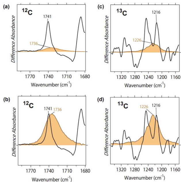
Fig. 5 (a) Spectral comparison of the C=O stretch of ACh in M_2R (black line) and in aqueous solution (orange line). The concentration of ACh is 1\text{ mM} in both cases. (b) Normalized peaks of the C=O stretch of ACh in M_2R (black line) and in aqueous solution (orange line), where the orange band was multiplied by 7.5. (c) Spectral comparison of the C–O stretch of ACh in M_2R (black line) and in aqueous solution (orange line). Concentration of ACh was 1\text{ mM} in both cases. (d) Normalized peaks of the C–O stretch of ACh in M_2R (black line) and in aqueous solution (orange line), where the orange band was multiplied by 3.3.
