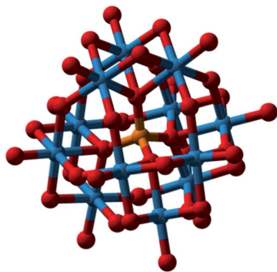
Fig. 14 Phosphotungstate anion [\text{PW}_{12}\text{O}_{40}]^{3-} . O, red; P, orange; W, blue. A central tetrahedral \text{PO}_4 surrounded by 12 octahedral \text{W}(\text{vi})\text{O}_6 , with bridging and terminal surface oxygens. This is the major component of phosphotungstic acid at pH 1. It is used in histology for staining of cells; it binds to fibrin, collagen, and connective tissues. Reproduced from https://en.wikipedia.org/wiki/Phosphotungstic_acid with permission from author (Benjah-bmm27).
