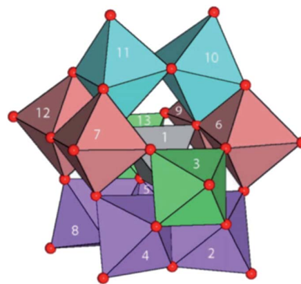
Fig. 15 Structure of [\text{Al}_{13}\text{O}_4(\text{OH})_{24}(\text{H}_2\text{O})_{12}]^{7+} in its sulfate salt. A central \text{Al}(\text{O})_4 unit surrounded by four trimeric groups of edge-shared \text{Al}(\text{O})_6 octahedra. Red, O; H atoms omitted. Reprinted with permission from Inorg. Chem. 2016, 55, 12270–12280. Copyright 2016 American Chemical Society. 97
