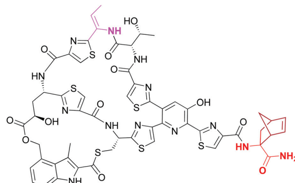
Scheme 24 Selective [2 + 4]-cycloaddition in nosiheptide by Roelfes et al. 83b
