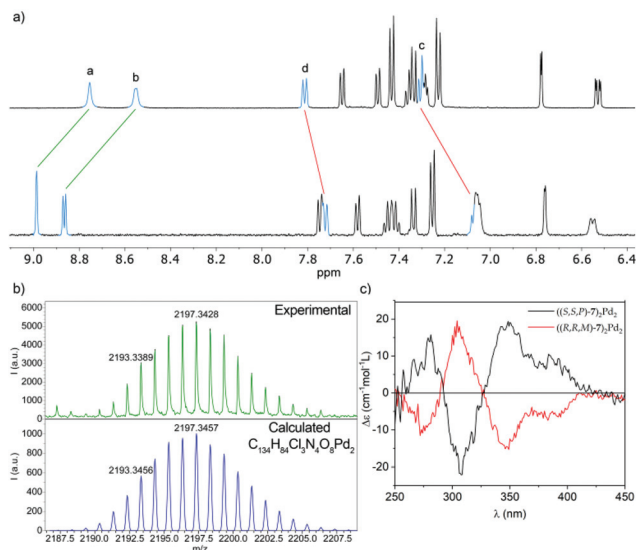
Fig. 9 (a) Partial 1 H NMR (500 MHz, CD 2 Cl 2 ) spectra of ligand ((S,S,P)-7) (top) and metallocyclic complex ((S,S,P)-7) 2 Pd 2 (bottom). The lettering corresponds to that shown in Fig. 1; (b) observed (top) and calculated (bottom) HRMS (MALDI + ) isotopic pattern for the [M - Cl] + ion of metallocyclic complex ((S,S,P)-7) 2 Pd 2 ; (c) ECD spectra of complex ((S,S,P)-7) 2 Pd 2 (black line) and its enantiomer ((R,R,M)-7) 2 Pd 2 (red line).
