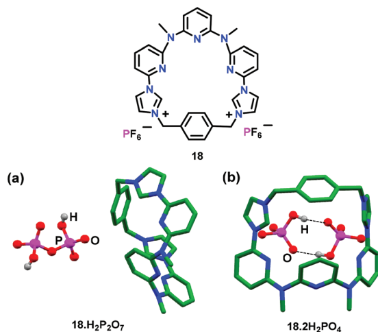
Fig. 8 Chemical drawing of chemosensor 18 . Crystal structures of (a) 18 \cdot \text{H}_2\text{P}_2\text{O}_7 and (b) 18 \cdot 2\text{H}_2\text{PO}_4^- . Hydrogen atoms except for phosphate anions have been excluded for clarity. Adapted from ref. 50.
