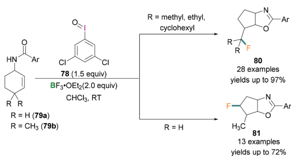
Scheme 32 Ring-contraction monofluorination reactions using \lambda^3 -iodanes ( 78 ) and Lewis acidic boranes.
