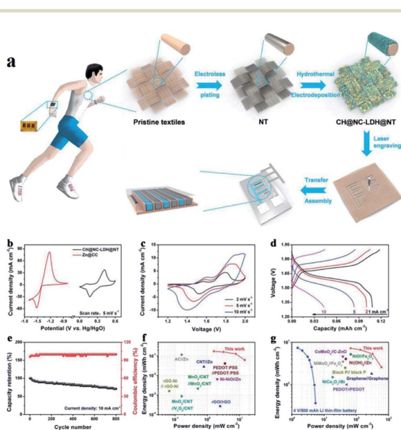
Fig. 2 (a) Fabrication process of Co-Zn alkaline microbattery. (b) Cyclic voltammograms of CH@NC-LDH@NT and Zn@CC at 5 mV s -1 . (c) Cyclic voltammograms, (d) galvanostatic charge/discharge curves, (e) long-term cycling stability, and (f and g) Ragone plots of Co-Zn alkaline MB. Reproduced with permission. 27 Copyright 2020, Wiley-VCH.
