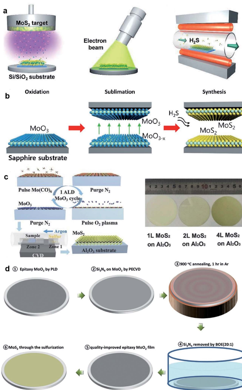
Fig. 4 (a) Schematic illustration of the synthetic process of the \text{MoS}_2 film: sputtering, EBL treatment, and sulfurization; 47 reproduced with permission from ref. 47, copyright 2020 American Chemical Society. (b) Schematic illustrations of the reaction sequence of monolayer \text{MoS}_2 via proximity evaporation of the Mo film precursor with the three steps (oxidation, sublimation, and synthesis); 49 reproduced with permission from ref. 49, copyright 2020 American Chemical Society. (c) Schematic of one cycle ALD process for the \text{MoO}_3 film and the sulfurization process for \text{MoS}_2 , and the photo of the \text{MoS}_2 film on a 2-inch sapphire wafer; 52 reproduced with permission from ref. 52, copyright 2017 John Wiley and Sons. (d) Flow diagram showing the synthesis of single-crystal \text{MoS}_2 films converted from CLAP-treated precursor \text{MoO}_2 films. 51 Reproduced with permission from ref. 51, copyright 2020 John Wiley and Sons.
