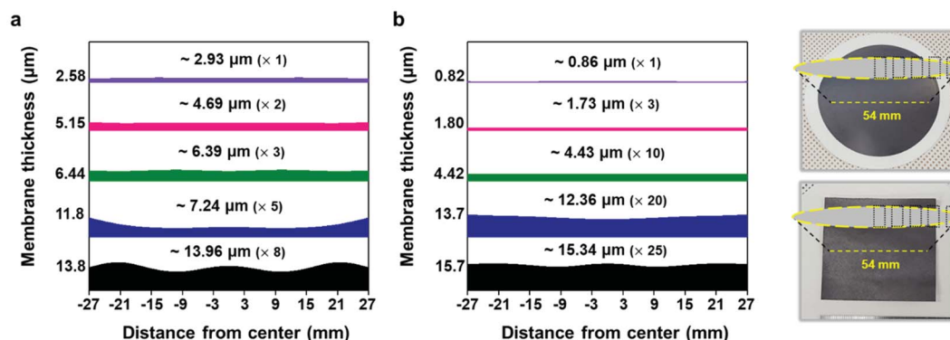
Fig. 5 Graph showing the cross-section thicknesses of the (a) vacuum-filtrated MXene membrane and (b) painted MXene ink. It shows the thickness non-uniformity of the MXene membrane deposited by two different ways over a large area of ≈54 mm in diameter. The numbers above the spectrum indicate the average thicknesses (the number of vacuum filtration or painting processes) of the MXene membranes. Photographs show the corresponding areas where the thicknesses were measured in the vacuum-filtrated MXene membrane (top) and painted MXene ink (bottom).
