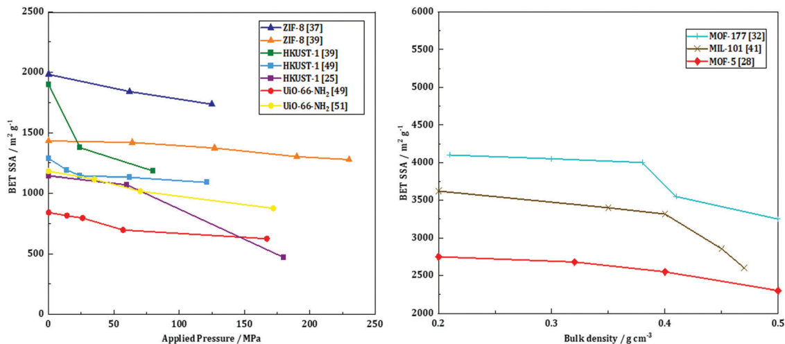
Fig. 3 BET SSA as a function of applied pressure during pelletization (left): ( \blacktriangle ) – ZIF-8 by Ribeiro et al. , 37 ( \blacktriangle ) – ZIF-8 by Bazer-Buchi et al. , 39 ( \bullet ) – UiO-66-NH 2 by Peterson et al. , 51 ( \bullet ) – UiO-66-NH 2 by Dhainaut et al. , 49 ( \blacksquare ) – HKUST-1 by Bazer-Buchi et al. , 39 ( \blacksquare ) – HKUST-1 by Dhainaut et al. , 49 and ( \blacksquare ) – HKUST-1 by Alcañiz-Monge et al. , 25 BET surface area as a function of bulk density (right): ( + ) – MOF-177 by Zacharia et al. , 32 ( \times ) – MIL-101 by Ardelean et al. , 41 and ( \blacklozenge ) – MOF-5 by Purewall et al. , 28
