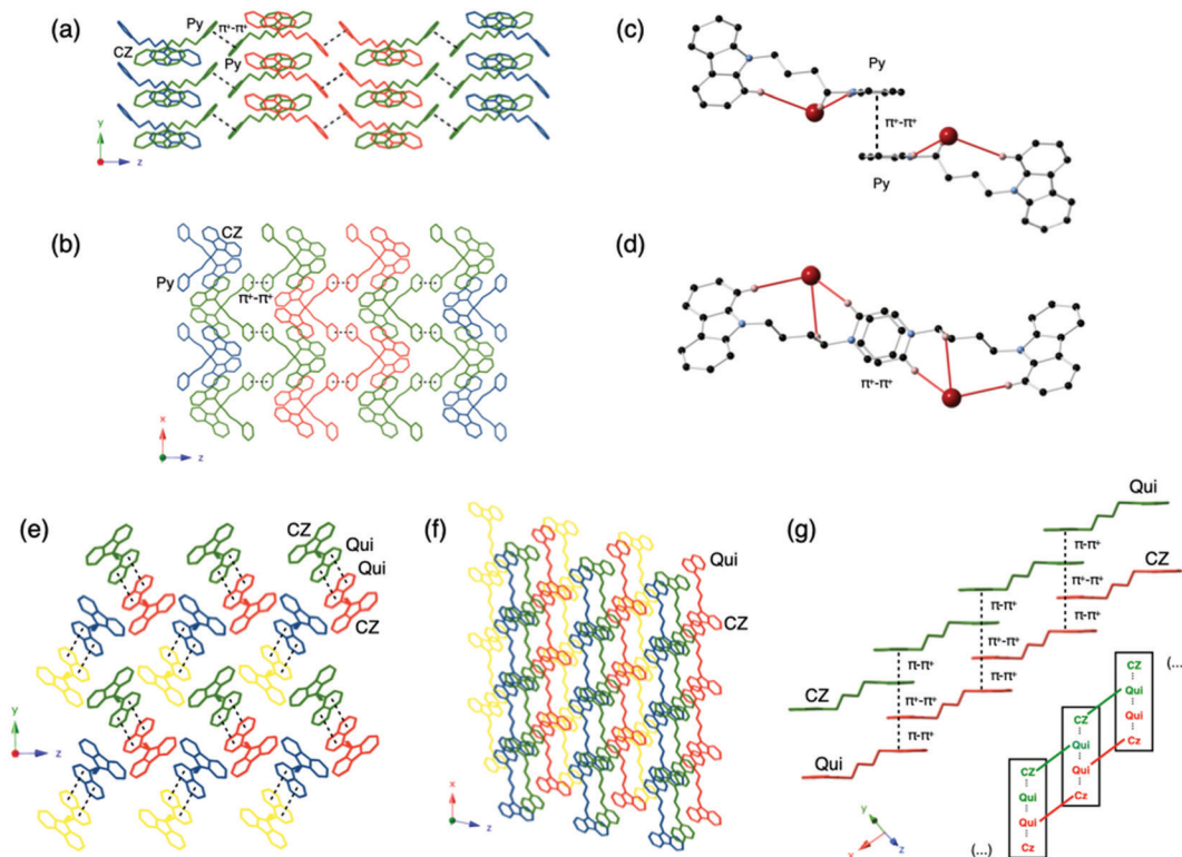
Fig. 1 Different crystal views of the intermolecular packing of Py-Br (a and b) and Qui-Br (e and f). (c and d) Molecular \pi^+\cdots\pi^+ and Br-H interactions in Py-Br . (g) Molecular \pi-\pi^+ and \pi^+\cdots\pi^+ interactions in Qui-Br .
