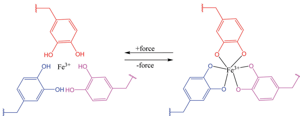
Fig. 8 Coordination bond between catechol ligands and Fe 3+ [reproduced from ref. 38 with permission from the Royal Society of Chemistry].
