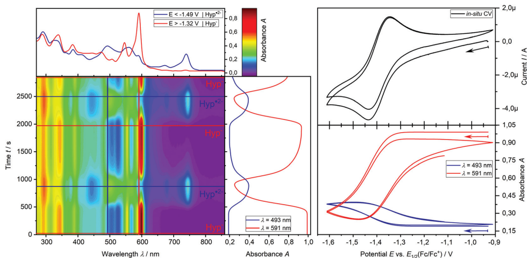
Fig. 7 In situ UV-vis-CV SEC measurement of hypericin (0.5 mM) in DMSO with 0.1 M [ ^n\text{Bu}_4\text{N} ] [ \text{BF}_4 ] at a platinum grid electrode in a double compartment cuvette cell ( d = 0.5 mm); left: 2D plot of UV-vis spectra during the CV measurement with the UV-vis spectra of \text{Hyp}^- (red) and \text{Hyp}^{2-} (blue); upper right: 2 cycles of CV; lower right: potential dependent absorbance at 591 nm (red) for \text{Hyp}^- and 493 nm (blue) for \text{Hyp}^{2-} .
