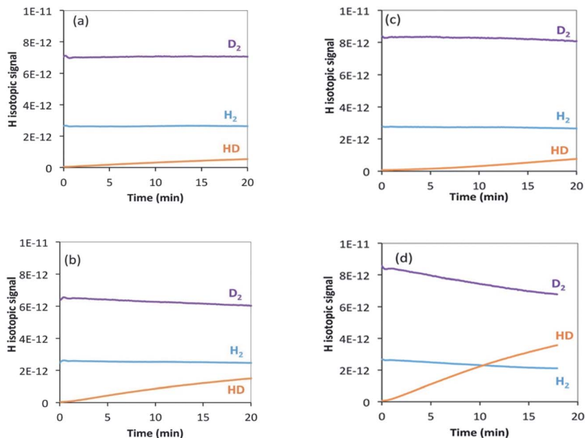
Fig. 7 \text{H}_2/\text{D}_2 exchange reaction on (a) \theta\text{-Mn}_6\text{N}_{5+x} at 200^\circ\text{C} , (b) \theta\text{-Mn}_6\text{N}_{5+x} at 250^\circ\text{C} , (c) 1% wt \text{Li}/\text{Mn}_6\text{N}_{5+x} at 200^\circ\text{C} , (d) 1% wt \text{Li}/\text{Mn}_6\text{N}_{5+x} at 250^\circ\text{C} .
