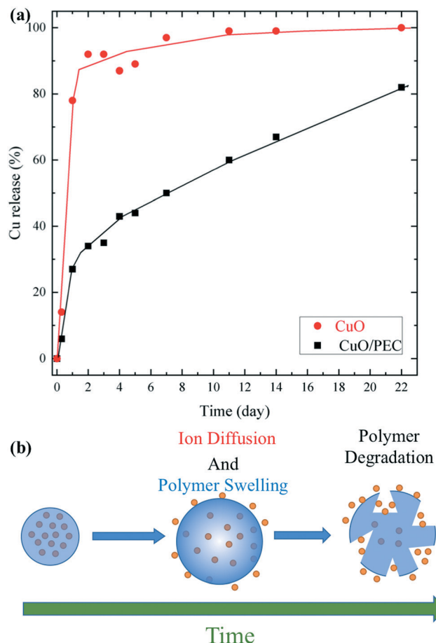
Fig. 6 (a) Cumulative percentage release of Cu versus time from CuO nanoparticles and the CuO/PEC NPs, under a constant of pH = 5.5. (b) Schematic of the mechanism of Cu release from the CuO/PEC nanocomposite.
