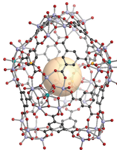
Fig. 33 Structural illustration of VMOP-22, \{[\text{V}_5\text{O}_9(\text{OCH}_3)]_4[\text{MoV}_5\text{O}_{11}(\text{SO}_4)]_4\}(\text{C1})_{12} . 161
