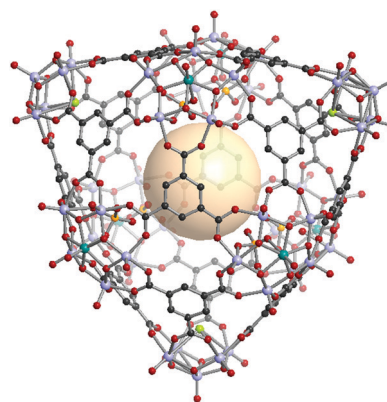
Fig. 34 Structural illustration of VMOP-23, \{[\text{V}_5\text{O}_9\text{Cl}]_3[\text{MoV}_5\text{O}_{11}(\text{SO}_4)]_6\}(\text{C1})_{14} . 161
