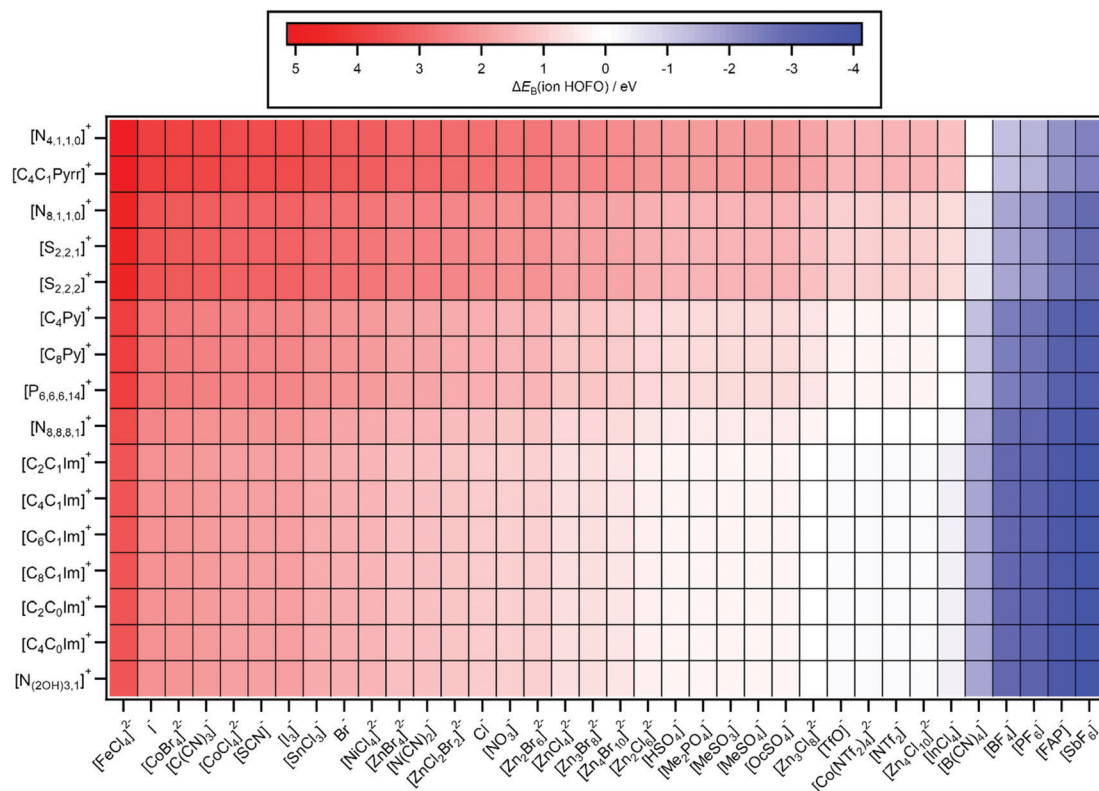
Fig. 7 Predicted \Delta E_B(\text{ion HOFO, pred.}) = E_B(\text{cation HOFO, pred.}) - E_B(\text{anion HOFO, pred.}) = E_i(\text{cation, pred.}) - E_i(\text{anion, pred.}) . The errors in \Delta E_B(\text{ion HOFO, pred.}) generally range from \pm 0.4 eV to \pm 0.6 eV.
