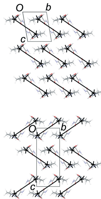
Fig. 4 Energy-vector models based on the stabilising interactions in FII and FIII. The diagrams look identical within the common 2-D layers (horizontal), but differ in orientation in neighbouring layers. Strong interactions are also formed along the a axis (perpendicular to the page) due to \text{N-H}\cdots\text{O} hydrogen bond between molecules within the polytypic layers.
