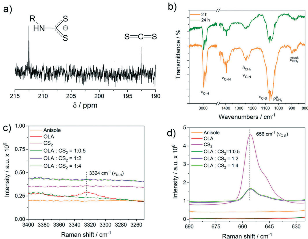
Fig. 4 (a) Low-field ^{13}\text{C} NMR spectrum of a solution of \text{CS}_2 (0.2 M) and oleylamine (0.129 M) in anisole. (b) FTIR of the particles synthesized at 250 °C. (c and d) Raman spectra in solution of pure anisole (5 mL), OLA (1 mL, 3 mmol in 5 mL anisole), and \text{CS}_2 (800 \mu\text{L} , 13 mmol in 5 mL anisole) and of anisole solutions of OLA (always 1 mL in 5 mL anisole) and various volumes of \text{CS}_2 : 90 \mu\text{L} (1.49 mmol), 360 \mu\text{L} (5.96 mmol), and 800 \mu\text{L} (13 mmol) corresponding to OLA : \text{CS}_2 ratio of 1 : 0.5, 1 : 2 and 1 : 4 mol : mol, respectively.
