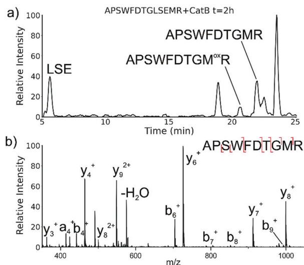
Fig. 2 (a) LC chromatogram for the incubation of APSWFDGLSEMR with catB. The labelled fragment APSWFDGLSEMR is produced by protease cleavage first followed by ligation of the dipeptide MR onto the proteolytic fragment APSWFDGL. (b) CID fragmentation of the ligated peak APSWFDGLSEMR.
