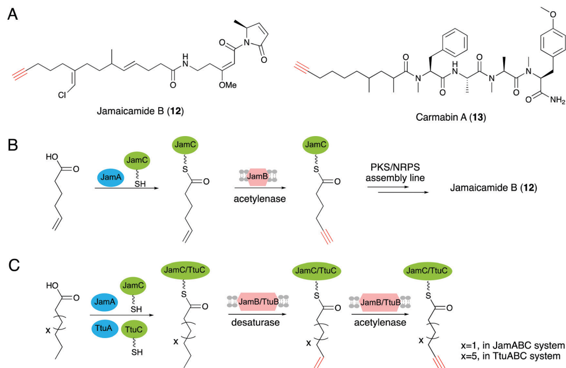
Fig. 6 (A) Structures of 12 and 13 . (B) The biosynthetic pathway for the C6 alkyne unit generation and incorporation into jamaicamide B. (C) Terminal alkyne biosynthetic pathways of JamABC and TtuABC that modify C6 and C10 fatty acids, respectively.
