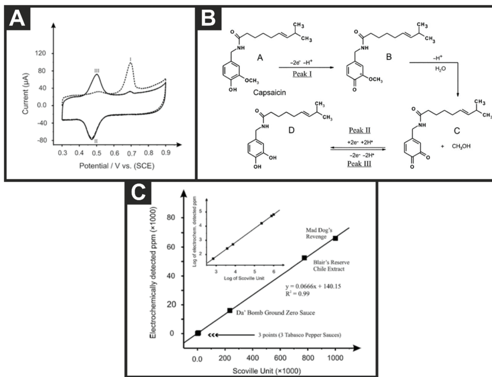
Fig. 2 (A) The first (dotted lines) and second (solid line) scans for the AdSV of 100 µM capsaicin on the MWCNT-BPPGE in a 0.05 M Britton–Robinson buffer solution at pH 1.0, after 1 min accumulation in open circuit conditions; scan rate: 100 mV s -1 . (B) Proposed electrochemical mechanism for the electrochemical oxidation/reduction of capsaicin. (C) Measured value of capsaicin concentration in ppm (electrochemically detected ppm) versus the average Scoville units for six hot pepper sauces. Inset: log of the electrochemically detected ppm versus log of the average Scoville units for six hot pepper sauces. Scheme and images reproduced with permission from ref. 40. Copyright Royal Society of Chemistry 2008. 40
