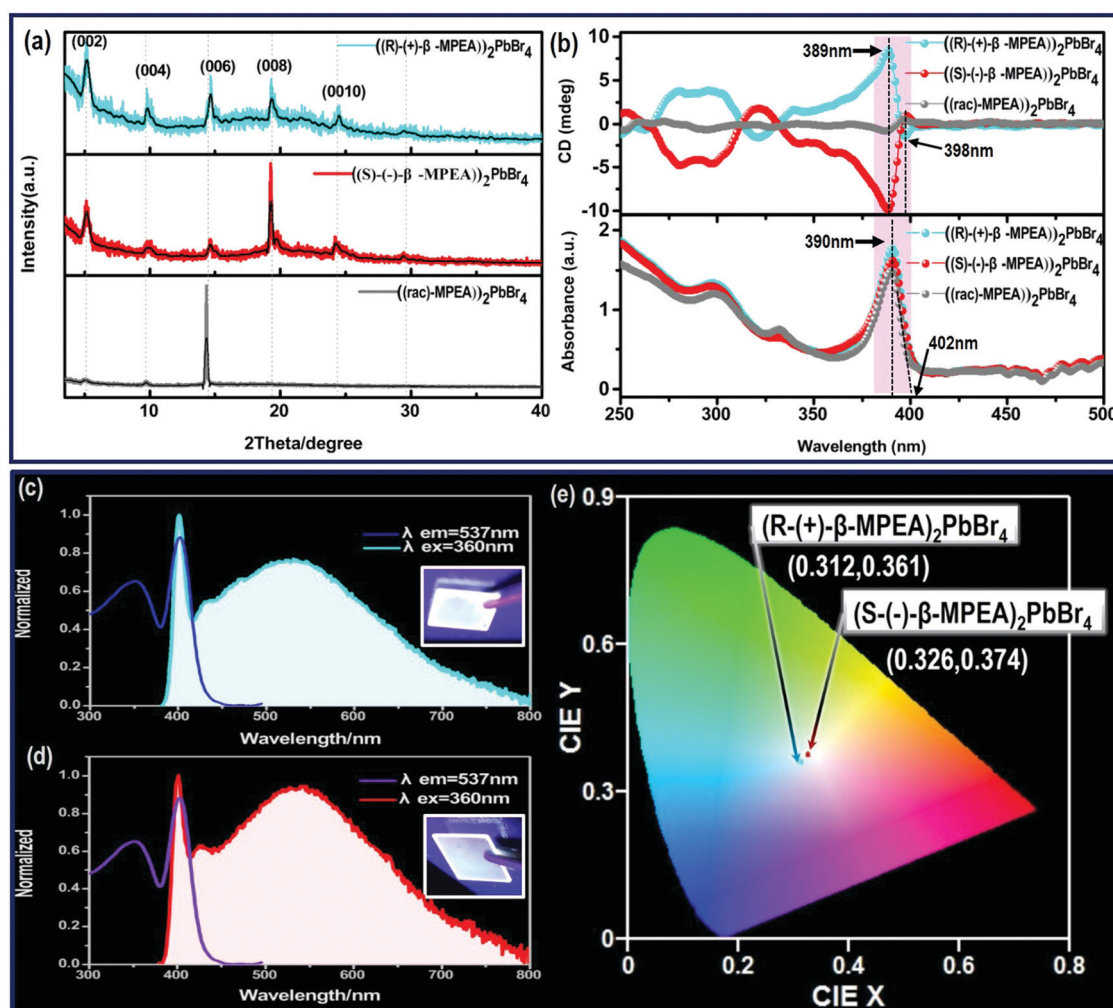
Fig. 2 (a) The XRD patterns of chiral perovskite crystals ( R -(+)- \beta -MPEA) 2 PbBr 4 , ( S -(-)- \beta -MPEA) 2 PbBr 4 film, ( rac -MPEA) 2 PbBr 4 film, (b) circular dichroism and steady-state absorption spectra of these perovskite crystals film. (c) PL and PLE spectra of ( R -(+)- \beta -MPEA) 2 PbBr 4 and ( S -(-)- \beta -MPEA) 2 PbBr 4 film ( \lambda_{\text{ex}} = 360 nm, \lambda_{\text{em}} = 537 nm), (d) PL and PLE spectra of ( S -(-)- \beta -MPEA) 2 PbBr 4 and ( S -(-)- \beta -MPEA) 2 PbBr 4 film ( \lambda_{\text{ex}} = 360 nm, \lambda_{\text{em}} = 537 nm), (e) CIE coordinated of the emissions of ( R -(+)- \beta -MPEA) 2 PbBr 4 and ( S -(-)- \beta -MPEA) 2 PbBr 4 film.
