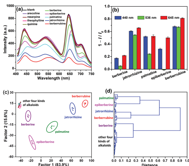
Fig. 3 (a) Fluorescence spectra of TCPP 0.09 Uio-66-(NH 2 ) 0.62 (diOH) 0.38 (50 mg L -1 ) after the addition of alkaloids (50 μM). (b) Intensity changes of the three emission bands upon exposure to berberine homologues. (c) LDA and (d) HCA plots for the discrimination of berberines.
