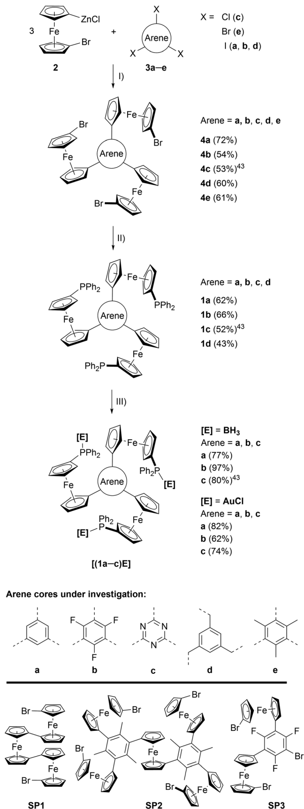
Scheme 1 (Top) Preparation of tris-phosphanes 1a–d and complexes [(1a–c)E] . (II) Pd precatalyst, THF, r. t.; (III) n BuLi, Ph 2 PCL, THF, –80 °C to r. t.; (III) [E]·X ([E]·X = BH 3 ·SMe 2 or [AuCl(ths)], CH 2 Cl 2 , r. t.; (Bottom) crystallographically characterised side products obtained during the syntheses of 4d (SP1), 4e (SP2), and 4b (SP3). For their solid-state structures, see Fig. S3.†
