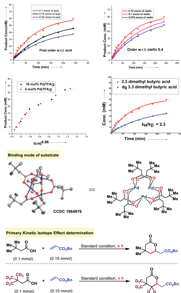
Fig. 7 Mechanistic investigation.
