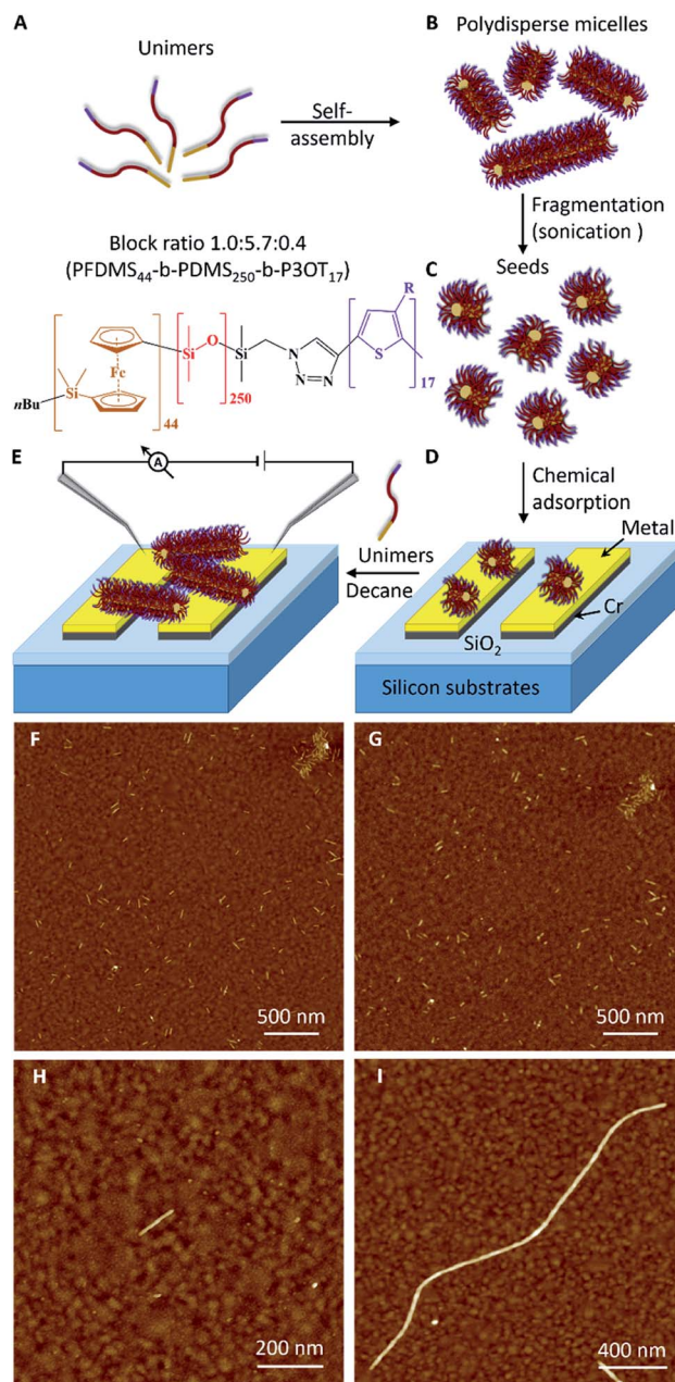
Fig. 1 Growth of fibre-like micelles via the living crystallisation-driven self-assembly of PF 44 b -PD 250 b -P 30T block terpolymers. (A) Schematic representation of the formation of cylindrical micelles. The chemical structure of unimers are shown in orange (PF 44 ), red (PDMS) and purple (P 30T ). (B) Self-assembly of PF 44 b -PD 250 b -P 30T unimers to form polydisperse micelles. (C) Fragmentation of the micelles using sonication to yield seeds. (D) Chemical adsorption of seeds on a metal (Au or Pt) electrode surface. (E) Growth of a fibre-like micelle from adsorbed seeds to cross the inter-electrode gap of an electrical device. (F and G) AFM images of adsorbed seeds on gold surface after immersion for 2 h in a 0.5 \mu g ml -1 solution in decane. The surfaces were then washed by immersion for (F) 2 min and (G) 24 h in pure decane. (H) Image of a seed adsorbed on a gold substrate from a 0.005 \mu g ml -1 solution of seeds immersed for 2 h. (I) Image of a micelle grown from an adsorbed seed on gold by immersion in a 4 \mu g ml -1 solution of unimers for 18 h.
