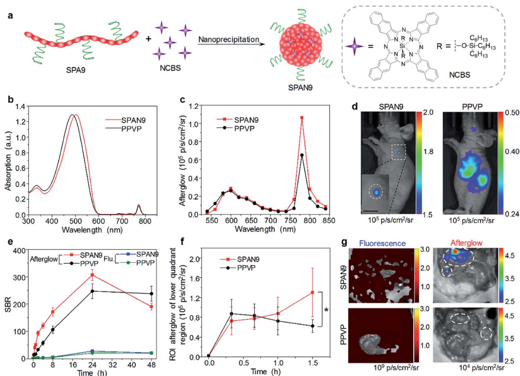
Fig. 3 (a) Schematic illustration for the preparation of SPAN9. (b) Absorption spectra of SPAN9 and PPVP in 1\times PBS buffer (pH 7.4). (c) Afterglow spectra of SPAN9 and PPVP under the same mass concentration ( 130 \mu\text{g mL}^{-1} ). (d) Afterglow images of living mice after i.v. injection of SPAN9 or PPVP for 40 min. (e) SBRs for fluorescence and afterglow imaging of tumor in living mice injected with SPAN9 or PPVP as a function of post-injection time. (f) Afterglow intensities of the lower quadrant region of living mice after i.v. injection of SPAN9 or PPVP as a function of post-injection time. (g) Fluorescence and afterglow images of abdominal cavity of mice after skin resection at 1.5 h post-injection of SPAN9 or PPVP. White circles mark the position of tumors. *Statistically significant difference ( p < 0.05 , n = 3 ). Error bars represent standard deviations of three different measurements ( n = 3 ). Adapted from ref. 93. Copyright© 2018 Wiley-VCH Verlag GmbH & Co. KGaA, Weinheim.
