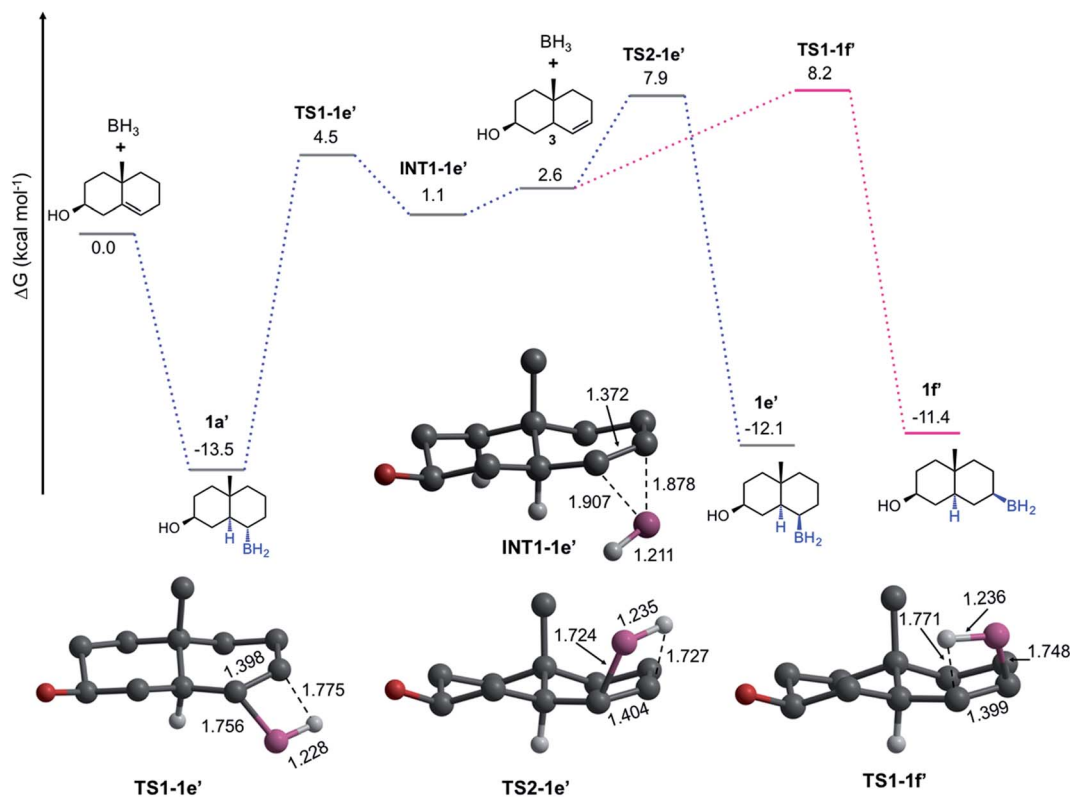
Fig. 4 Gibbs energy profiles (in \text{kcal mol}^{-1} ) for the formation of 1e' and 1f' and transition state structures involved. Bond distances are in Å. In the depicted structures, H atoms are omitted for clarity, except the H atom involved in the hydroboration.
