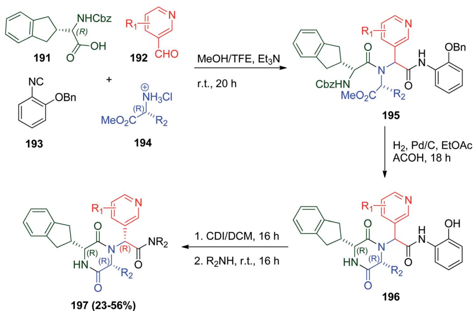
Scheme 41 Synthesis of epelsiban derivatives 197 via Ugi reaction.
