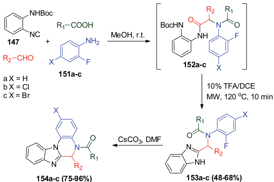
Scheme 32 Synthesis of fused benzimidazole-quinoxalones 154a-c via UDC reaction.
