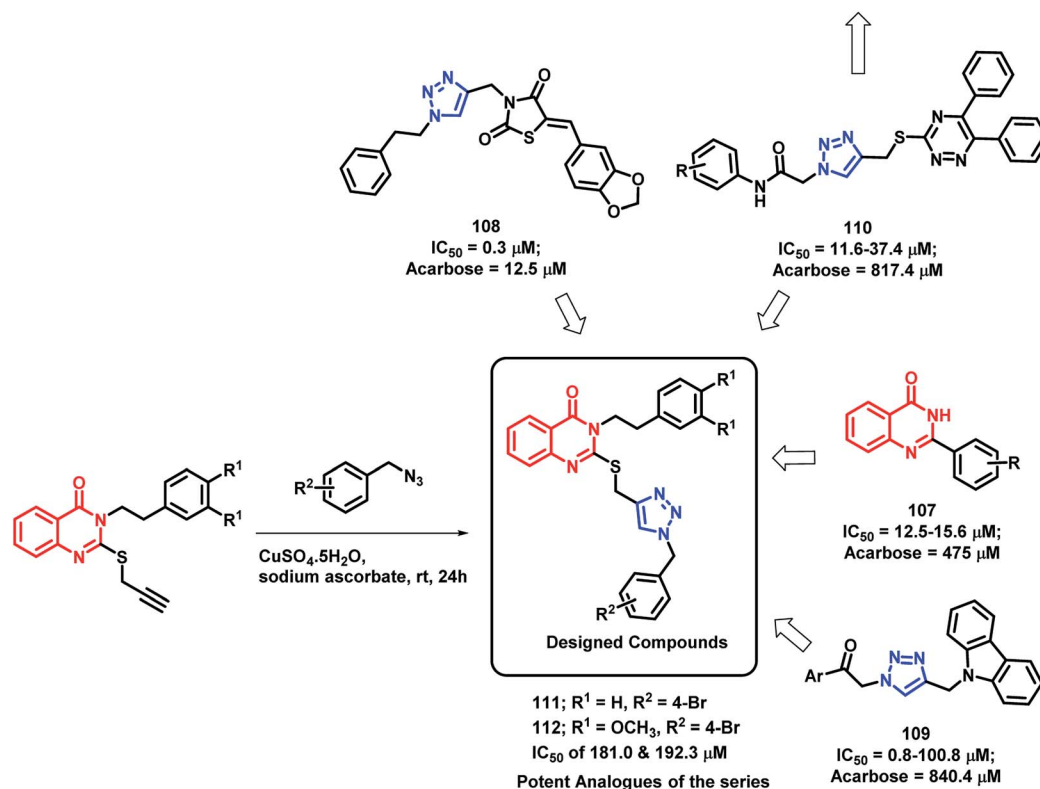
Scheme 41 Synthesis and design strategy for triazole-linked quinazolinone hybrids, targeting \alpha -glucosidase.
