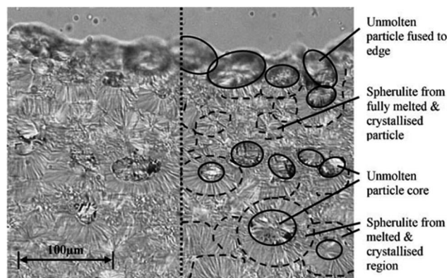
Fig. 6 Optical microscopy image displaying the crystal structure of PA 12. 45 Reprinted with permission from Elsevier: Materials Science and Engineering: A , Copyright 2019, License: 4838261169022.
