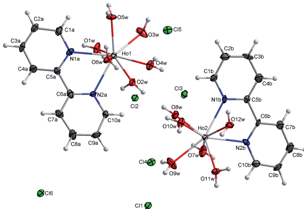
Fig. 2 An ORTEP view of the molecular structure of [\text{Ho}(\text{bpy})(\text{H}_2\text{O})_6]\text{Cl}_3 with ellipsoids drawn at the 50% probability level.
