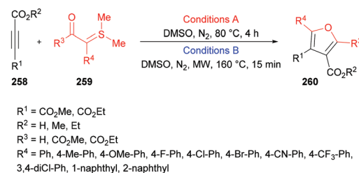
Scheme 67 Regiospecific synthesis of polysubstituted furans from sulfonium acylmethylenes and acetylenic esters.
