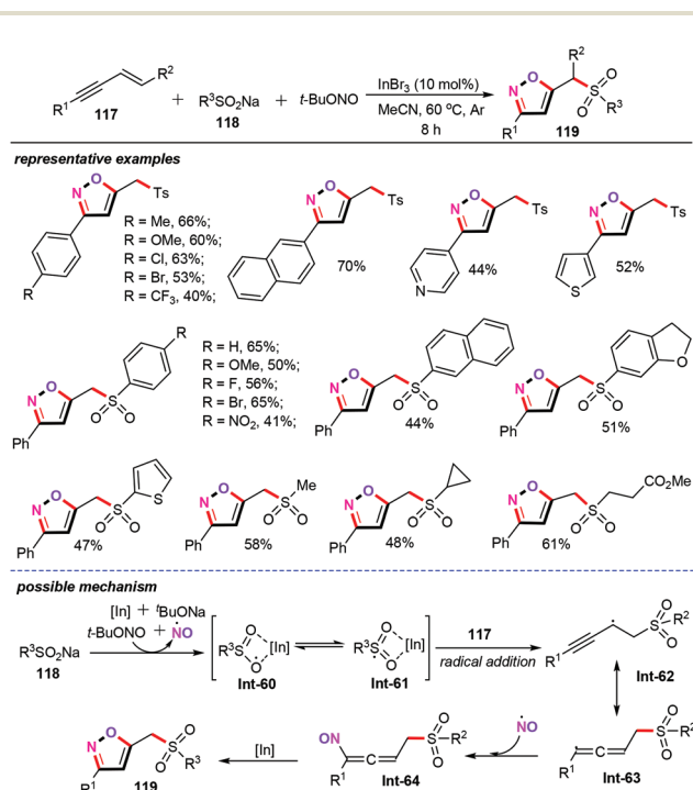
Scheme 48 Indium-catalyzed 1,3,4-trifunctionalization cascade of 1,3-enynes for the synthesis of 5-sulfonylisoxazoles.
