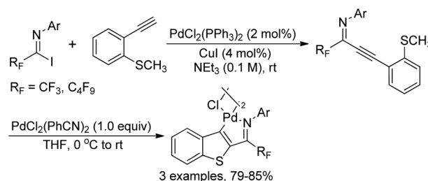
Scheme 38 Synthesis of benzothiophene-based palladacycles.
