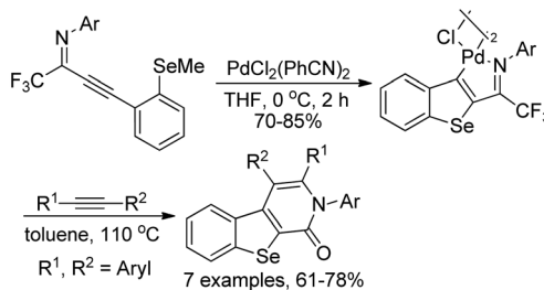
Scheme 42 Synthesis of cyclopalladated benzoselenophene.
