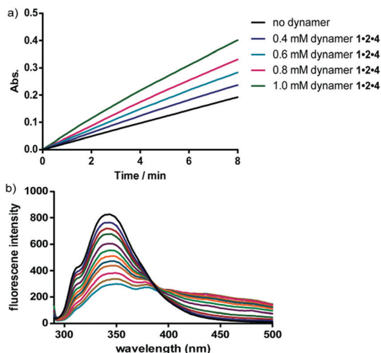
Fig. 12 (a) Representative UV time-course study of CA activity changes upon hydrolysis reaction of p -nitrophenyl acetate, showing increased activity by adding more dynamer 1.2.4 ; (b) representative fluorescent titration study for CA-dynamer 1.2.4 interactions, the fluorescence intensity was gradually quenched with increasing amount of dynamer 1.2.4 . 137 Copyright 2016 The Royal Society of Chemistry.
