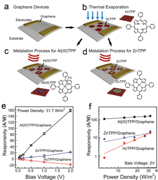
Fig. 10 (a-d) Schematic representation of H 2 TPP- and metalloporphyrin-graphene hybrid film formation. (e) Photoresponsivity of H 2 TPP-, ZnTPP-, and Al(III)TPP-graphene-based devices as a function of the source-drain bias voltage during exposure to light with a power density of 31.7 W m -2 . (f) Photoresponsivity as a function of the light power density; a bias voltage of 2 V was used for the measurements. Copyright 2016, Nanotechnology. 43
