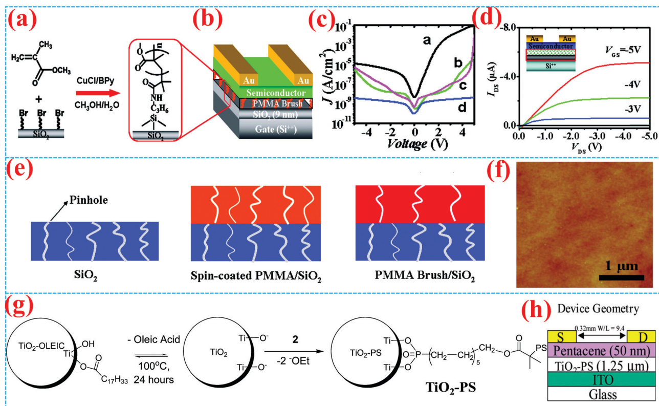
Fig. 4 (a and b) Schematic illustration of a surface-grafting PMMA brush on \text{SiO}_2 as a hybrid nanodielectric for OFETs. (c) Leakage characteristics for different dielectrics with the structure of Au/dielectric/Si capacitor. Curve a: 9 nm \text{SiO}_2 ; curve b: spin-coated PMMA (10 nm) and \text{SiO}_2 (9 nm); curve c: surface-grafting PMMA (20 nm); curve d: surface-grafting PMMA (10 nm) and \text{SiO}_2 (9 nm). (d) Transfer curves of pentacene OFETs with PMMA/ \text{SiO}_2 nanodielectrics. (e) Schematic diagram of distribution of pinhole defect. (f) AFM image of a PMMA brush. 25 Copyright 2010, American Chemical Society. (g) Synthetic route for \text{TiO}_2 -PS core-shell nanoparticles. (h) Schematic illustration of a pentacene OFET using 20 mol% \text{TiO}_2 -PS as the gate dielectric. 55 Copyright 2005, American Chemical Society.
