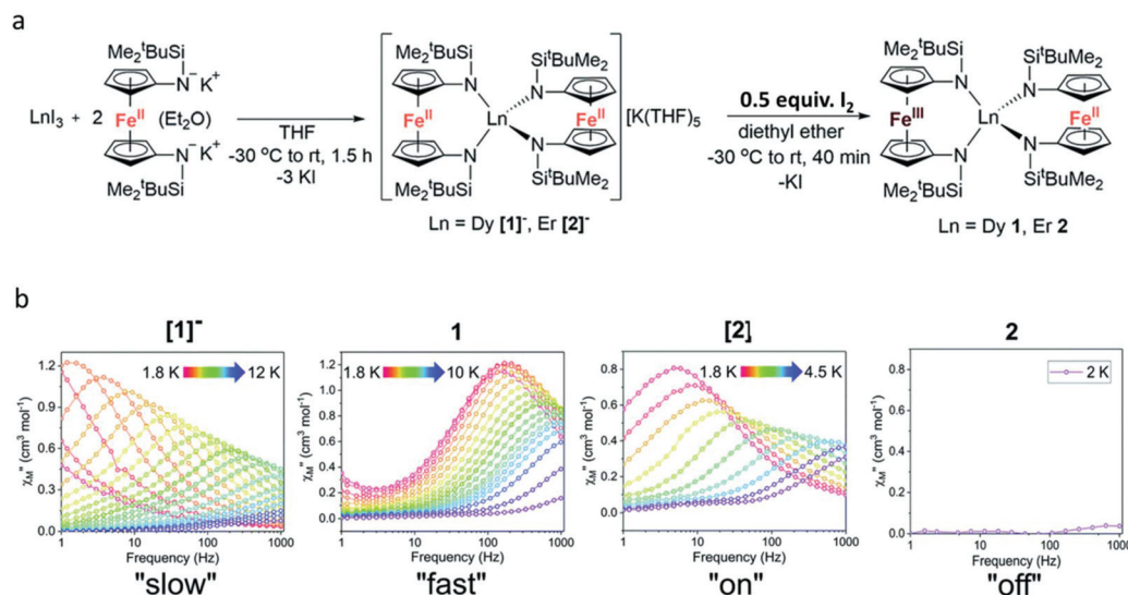
Fig. 8 (a) Synthesis of 1 ⁻, 1 , 2 ⁻, and 2 ; (b) plots of \chi''(\nu) for 1 ⁻ and 1 under a 1000 Oe dc field and 2 ⁻ and 2 under a 500 Oe dc field. Reproduced with permission from ref. 76. Copyright 2017 Royal Society of Chemistry. 76
