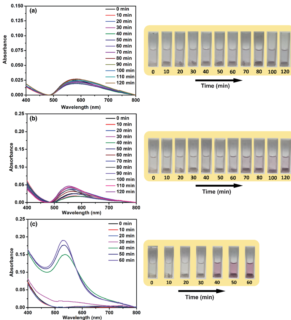
Fig. 5 Aggregation dynamics study of Au nanoclusters by monitoring the time-dependent UV-visible spectra of (a) ACA-0.25 (12 000 mg L -1 ), (b) ACA-1 (3000 mg L -1 ), and (c) ACA-6 (500 mg L -1 ) solutions. The panel on the right side shows the digital images of the corresponding solutions for visual observations. For the same aggregation dynamics studies, a 1000 mg L -1 of ACA-1 catalyst solution showed no visible color change by 120 min. Hence, the initial concentration of 3000 mg L -1 of ACA-1 catalyst solution was used.
