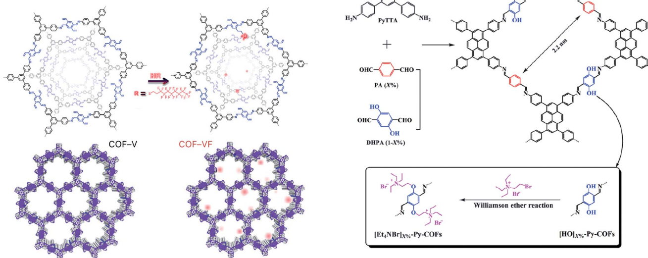
Fig. 46 Williamson ether synthesis of IL-functionalized [Et_4NBr]_{X\%}\text{-Py-COFs} for catalyzing the formylation reaction. Adapted with permission. 305 Copyright 2016, The Royal Society of Chemistry.
