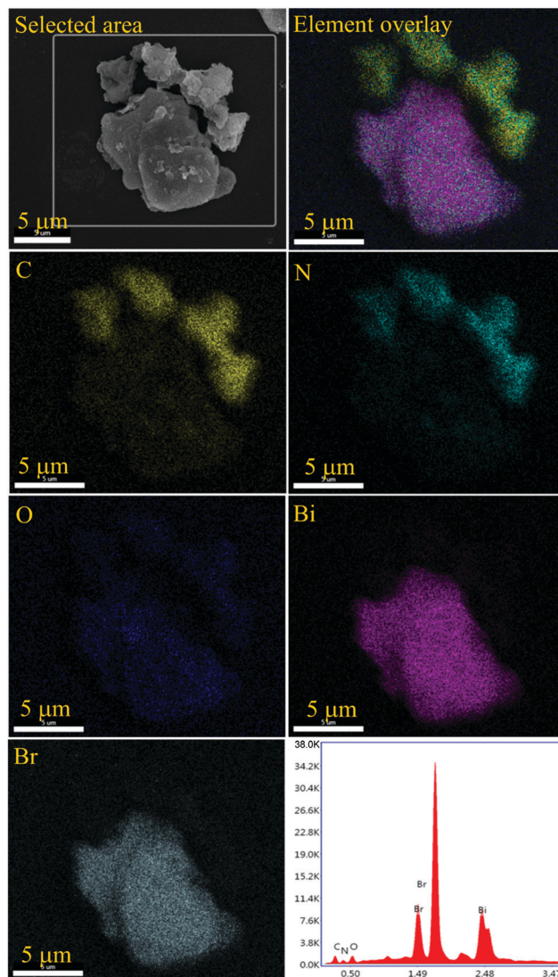
Fig. 5 Elemental mapping and EDAX spectrum of the BiOBr/g-C 3 N 4 composite.
